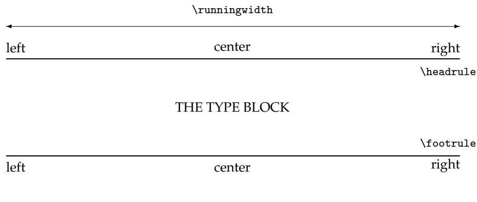
Figure 7.1: Header and footer slots
